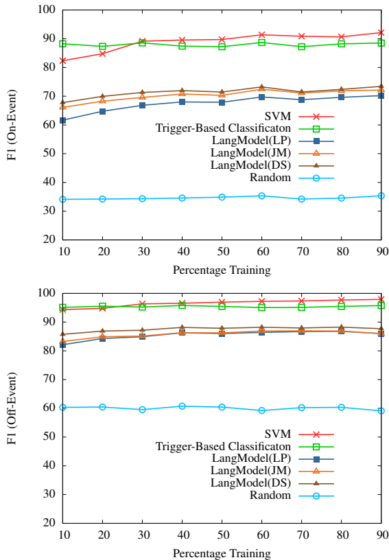
Figure 1: % F1 for the on-event (top) and off-event (bottom) classes for all methods using varying levels of training data where the target event is “Die”.
