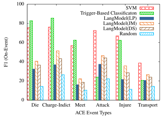
Figure 2: % F1 of the “on-event” class achieved by all methods for the six ACE event types.
