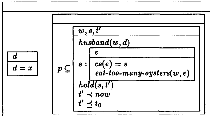
Figure 1: The SDRS representing Text (6)
