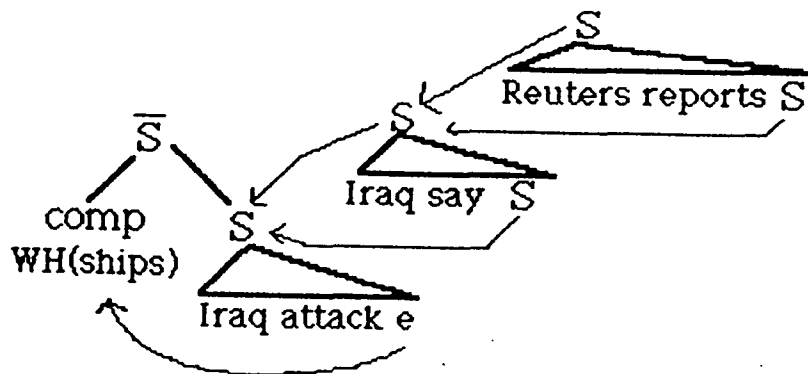
Figure 9 Question formation with sentential complement verbs
