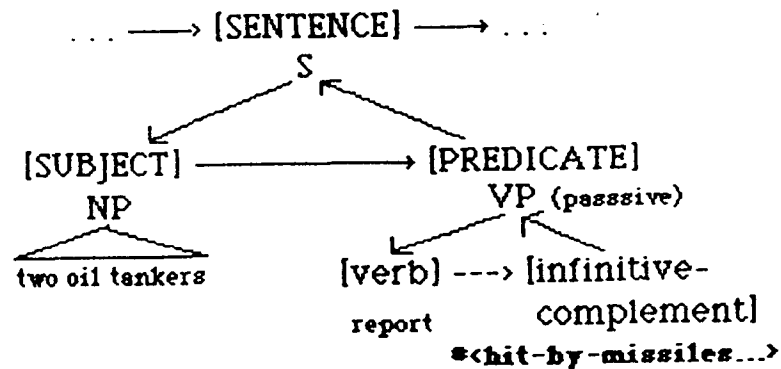
Figure 8 The path after attachment
