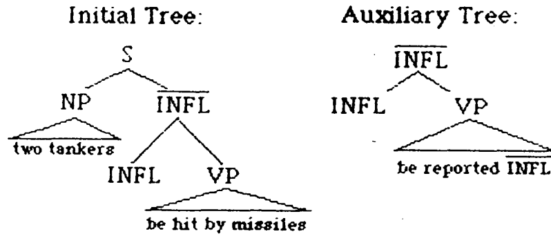
Figure 4 Initial and auxiliary trees for Raising-to-subject
