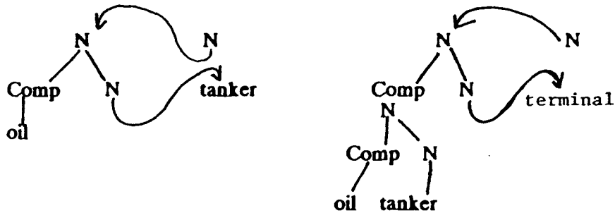
Figure 12 TAG Derivation of oil tanker terminal
