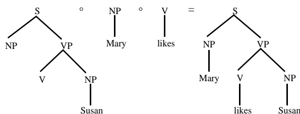
Figure 3. Another derivation yielding same tree
