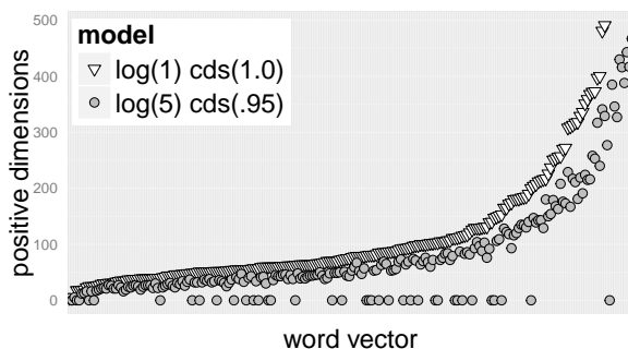
Figure 1: Along the X axis, vectors are ordered by the ascending number of positive dimensions in the vanilla model. The Y axis represents the number of positive dimensions in two models.
