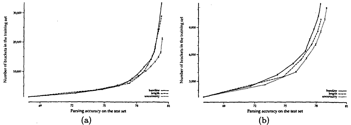
Figure 2: The learning rates of the induction processes using examples selected by the three evaluation functions for (a) when the candidate-pool is large, and (b) when the candidate-pool is small.
