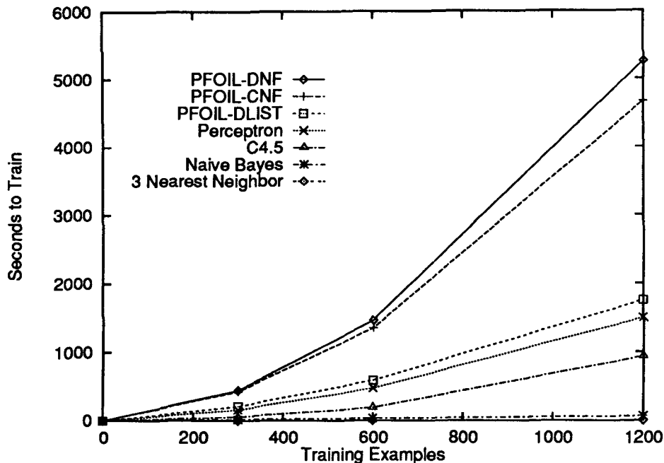
Figure 2: Training Time for "Line" Corpus
