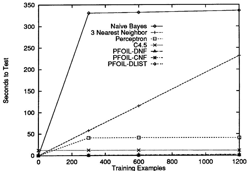
Figure 3: Testing Time for "Line" Corpus
