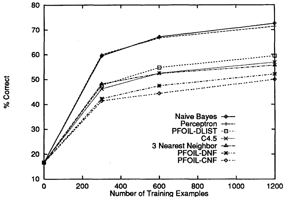
Figure 1: Accuracy at Disambiguating “Line”
