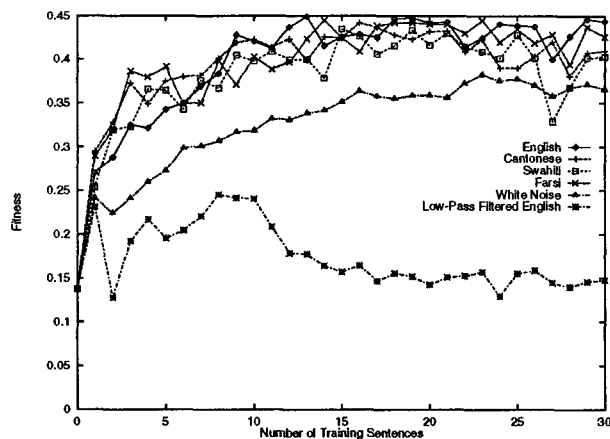
Figure 6: Network performance increases to its final value after presentation of just 20 sentences regardless of the language used to train the network. The six curves show the learning curves for a network tested on 30 sentences of English having been trained on English, Cantonese, Swahili, Farsi, white noise and low-pass filtered English.
