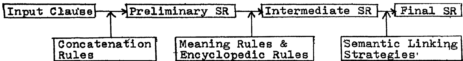
Fig.2: 3-Stage Model of Semantic Analysis
