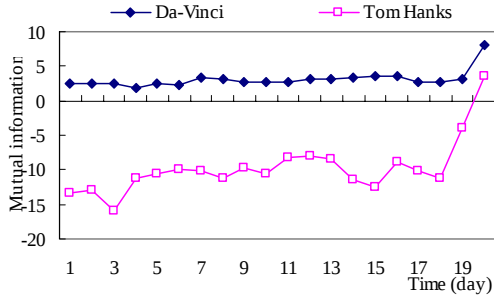
Figure 3: Interval-based Approach in Da Vinci Code
