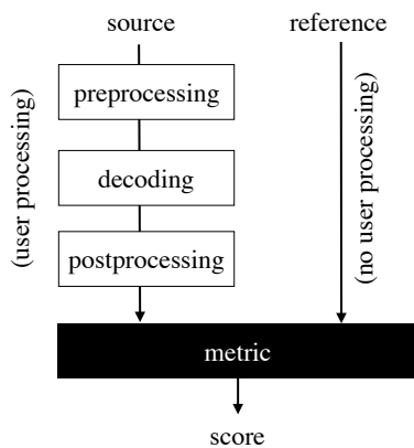
Figure 1: The proper pipeline for computing reported BLEU scores. White boxes denote user-supplied processing, and the black box, metric-supplied. The user should not touch the reference, while the metric applies its own processing to the system output and reference.
