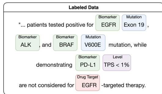
Figure 2: Snippet of our proprietary dataset.
