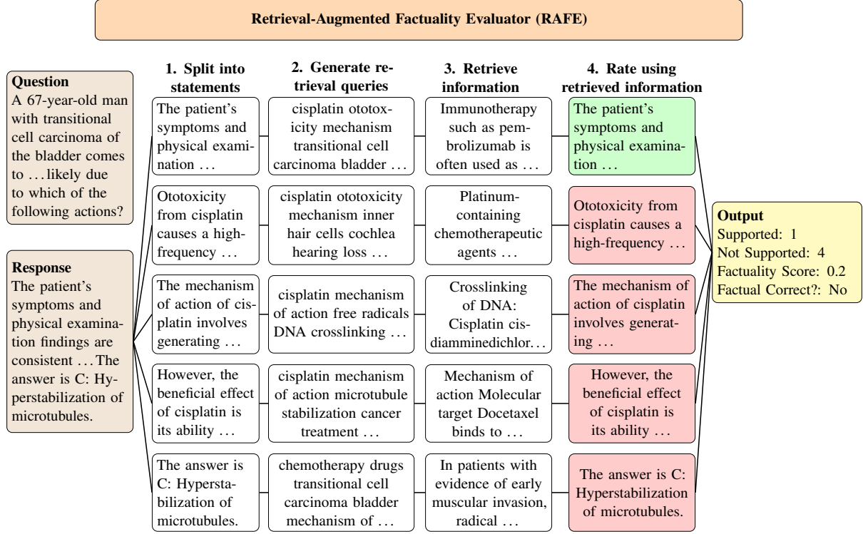
Figure 2: The Retrieval-Augmented Factuality Evaluator (RAFE) assesses the factual accuracy of response in four steps. (1) Split and rewrite statements: The response is divided into individual statements while preserving dependencies, and relevant statements are rewritten to be self-contained by incorporating necessary context. (2) Generate retrieval queries: For each statement, an LLM generates multiple context-aware retrieval queries that consider the original question and previously retrieved documents. (3) Retrieve information: The retrieval system performs multiple searches (three per statement) to progressively build comprehensive supporting evidence. (4) Rate using retrieved information: Each statement is evaluated against the accumulated evidence while maintaining awareness of the broader context, and labeled as Supported or Not Supported . The final output includes a factuality score, calculated as the proportion of supported statements, which aids in selecting the most factually reliable response.
