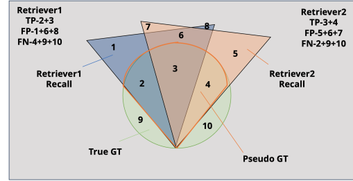
Figure 1: With our subset sampling method, we can get relative comparison between different retrievers.
