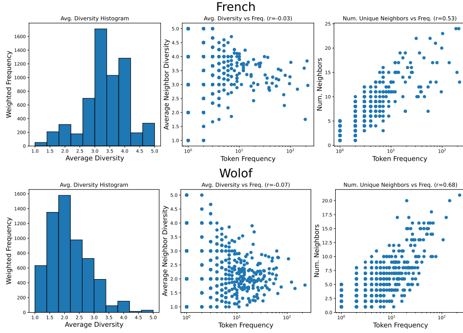
Figure 7: Case study results for French. Token frequency plotted using log scale. Pearson’s r is used. We also include Wolof, as it is a low-resource and unseen language. Details provided in Appendix D .
