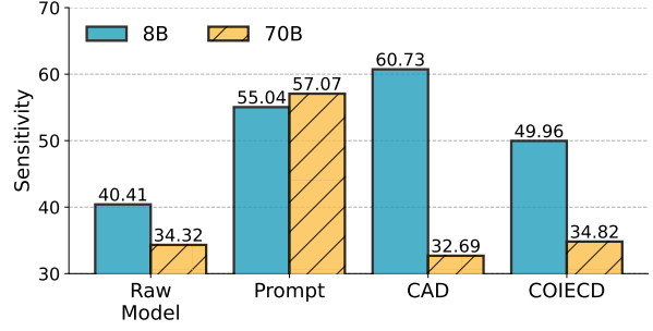
Figure 2: Performance of models of different sizes under different methods. The larger model tends to stick to its internal beliefs when faced with conflicting information. Prompting benefits both model sizes, while CAD and COIECD show excellent performance on the small model but provide minimal improvement for the large model.
