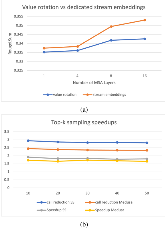
Figure 11: (a) We analyze the effect of value projection rotation on ROUGE LSum scores of the Dialog summarization task using OPT-1.3B as the base model for different numbers of MSA layers. Each stream is rotated in proportion to the distance from the main stream. (b) We study the effect of top-k sampling on wall-time speedups and call reduction ratios (mean tokens generated per step) for Speculative Streaming (SS) and Medusa-style approaches using OPT-1.3B as a base model on the Meaning Representation task.
