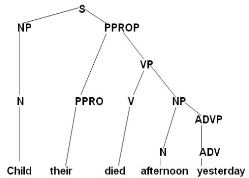
Figure IV: Parse tree showing conversion of possessive determiners from Igala to English.
