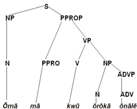
Figure 1: Parsing of inverse syntactic determiners in Igala.
