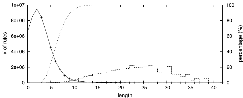
Figure 12 The solid-line curve represents the distribution of all rules against permutation lengths. The dashed-line stairs indicate the percentage of non-binarizable rules in our initial rule set, and the dotted line denotes that percentage among all permutations.
