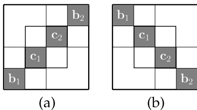
Figure 8 Illustration of the proof of Lemma 2. The arrangement of (b_1, c_1, c_2, b_2) must be either all straight as in (a) or all inverted as in (b).
