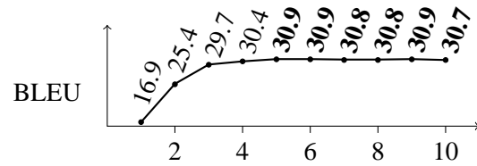
Figure 1: Effect of the maximum phrase length.
