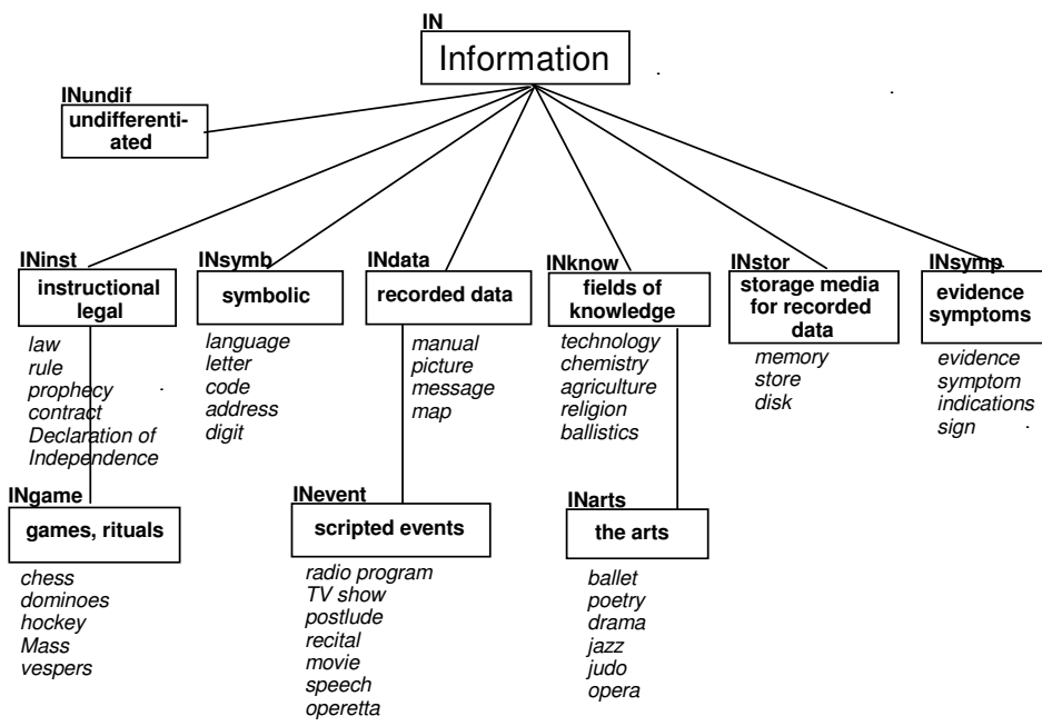
Figure 2: SAL Taxonomy for the Information Noun Superset with attending Sets and Subsets. Note that some Sets do not have Subsets.
