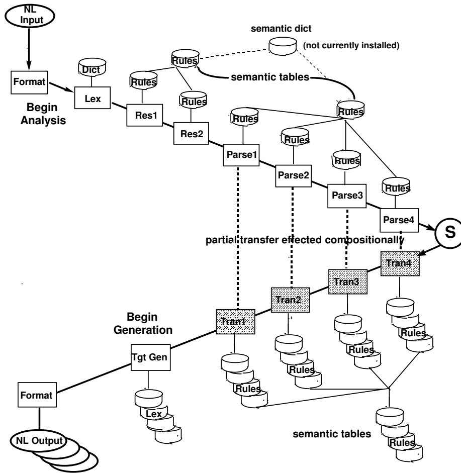
Figure 1: Modularized, Incremental Pipeline Architecture of OpenLogos
