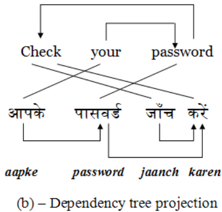
Figure 2: Projection of dependencies
