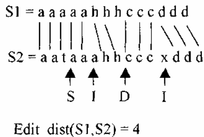
Figure 1. Edit Distance
