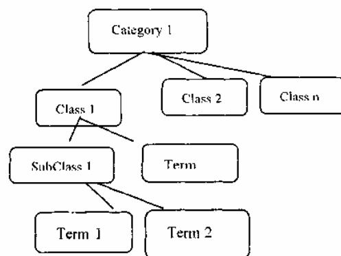
Figure 2. Thesaurus architecture
