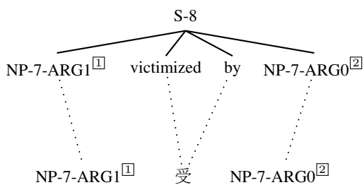
Figure 1: A complete semantic rule (Bazrafshan and Gildea (2013)).
