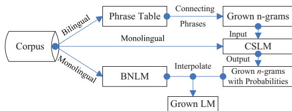
Figure 1: NN based bilingual LM growing.
