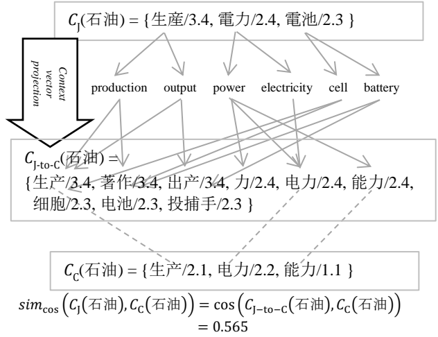
Figure 2. Calculation of contextual similarity by context-vector projection
