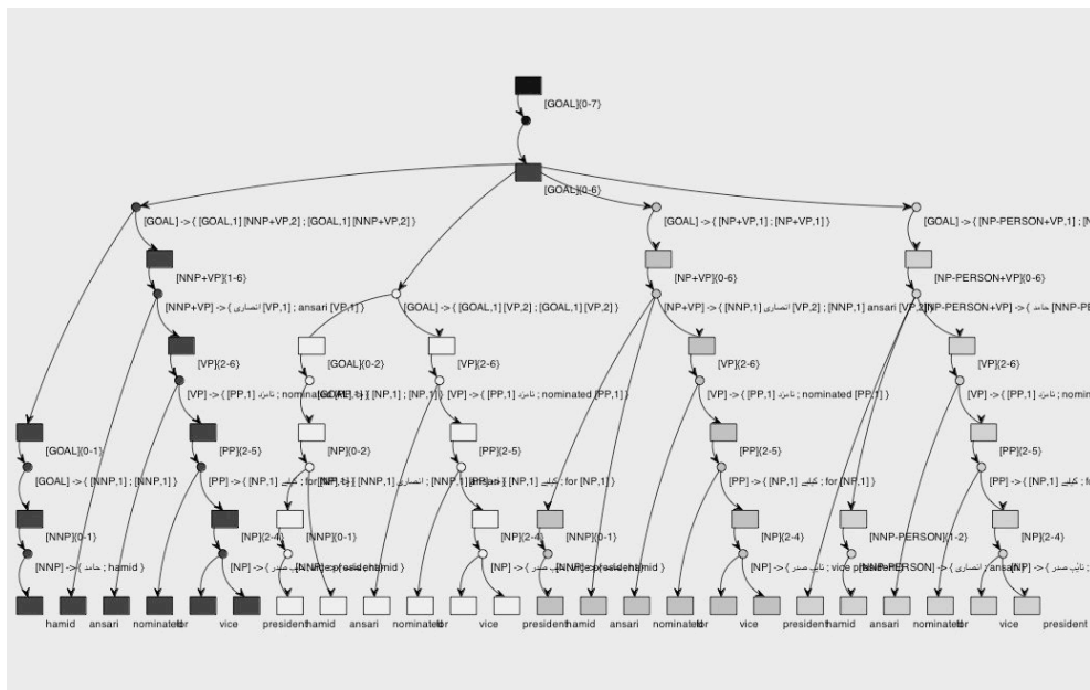
Figure 4. The visualization window for the hypergraph browser.
