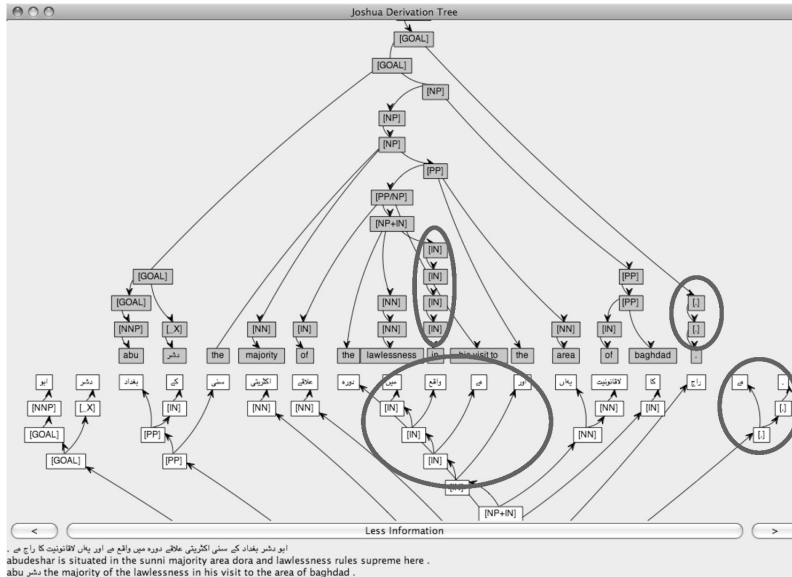
Figure 5. An example of bad production rules that parse pieces of the source sentence without producing any target-side output.
