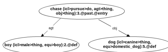
Figure 1: UNL Graph for 'The boy chased the dog'
