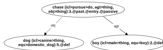
Figure 2: UNL Graph for 'The dog was chased by the boy'
