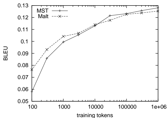
Figure 1: The effect of parser training data size of BLEU with Malt and MST parsers.
