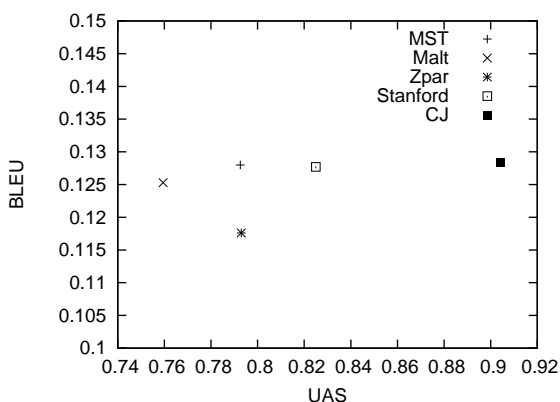
Figure 2: Unlabeled Attachment Score versus BLEU.
