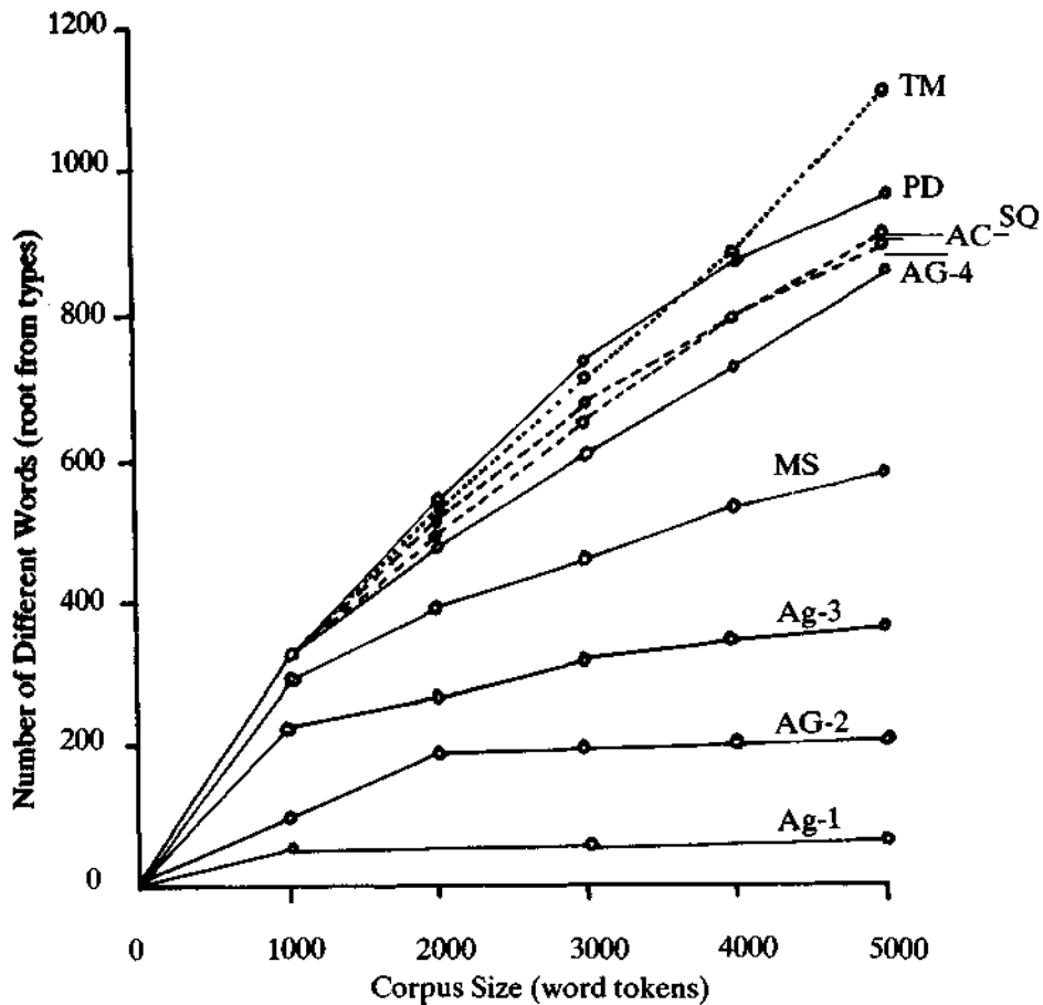
Figure 4. Comparison of vocabulary growth rate curves.
