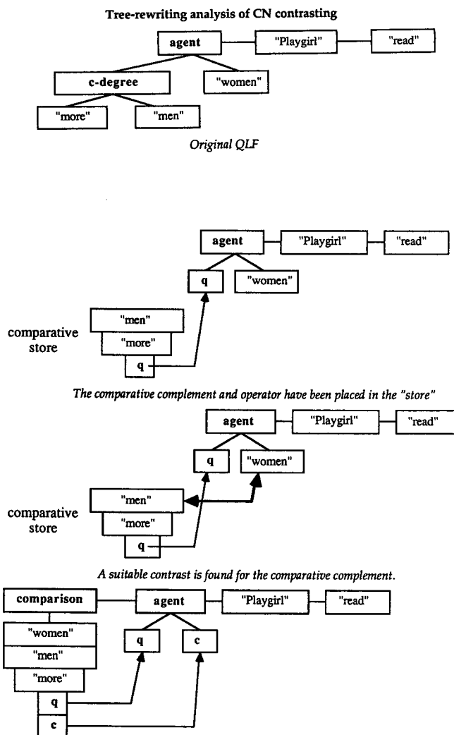
Figure 6 Tree re-writing analysis of CN-contrasting
