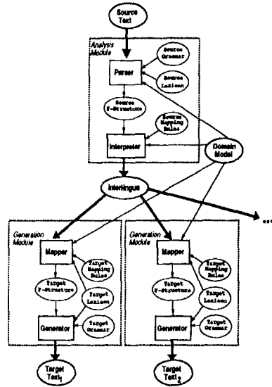
Figure 1: KANT: Knowledge-Based Natural Language Translation
