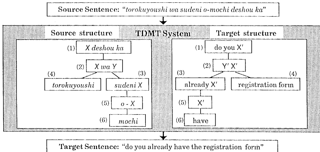
Fig. 4 A Transfer Example for “torokuyoushi wa sudeni o-mochi deshoushi ka”
