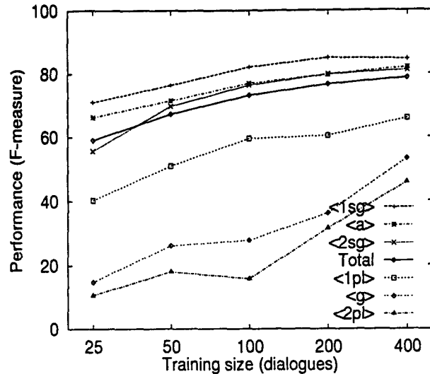
Figure 1: Training size and performance
