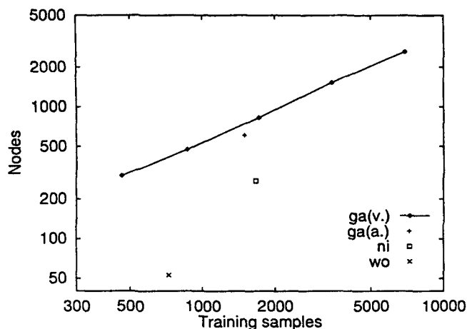
Figure 2: Training samples vs. nodes
