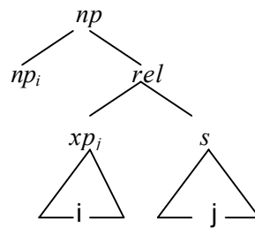
Figure 4: Relative clauses
