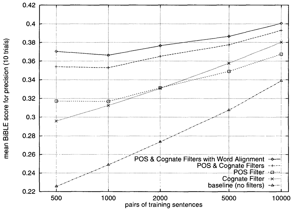
Figure 6: Each filter contributes to an improvement in BiBLE scores.
