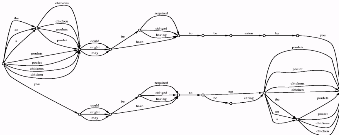
Figure 1: A small fragment of a sample Nitrogen word lattice. One path represents the fluent sentence you may have to eat chicken . Other paths correspond to less fluent or appropriate sentences. The full word lattice is many times larger than this fragment.
