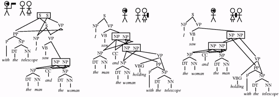
Figure 2: Three parse forests built from three semantic representations. The goal of ambiguity preservation is to identify the trees of just those sentences which cover all meanings.
