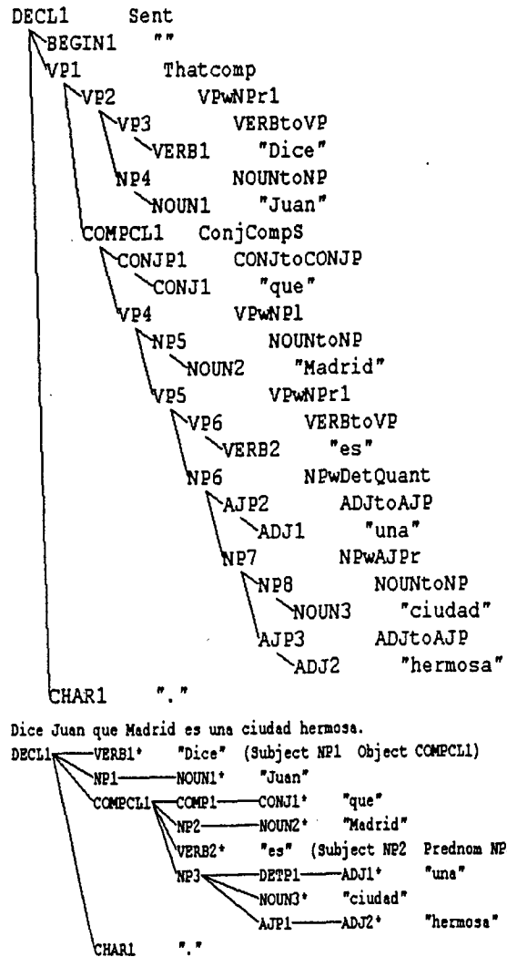
Figure 2: A derivational tree and a "flattened" tree for the sentence "Dice Juan que Madrid es una ciudad hermosa" ("John says that Madrid is a beautiful city")
