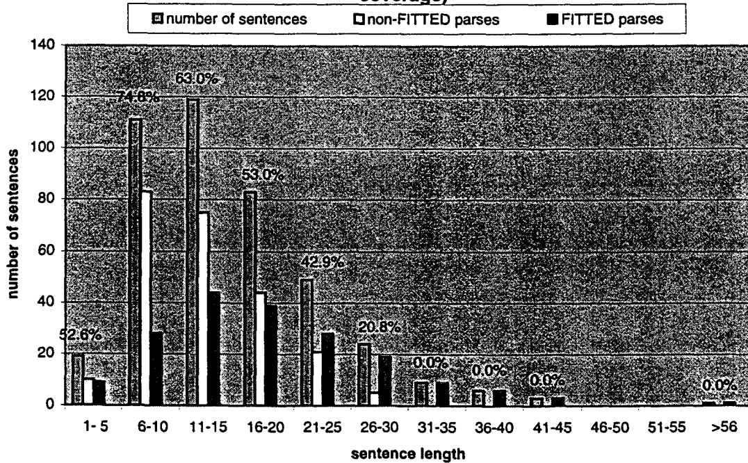
Figure 6: The number of non-FITTED parses versus FITTED parses in relation to sentence length for German (showing percentage of coverage)
