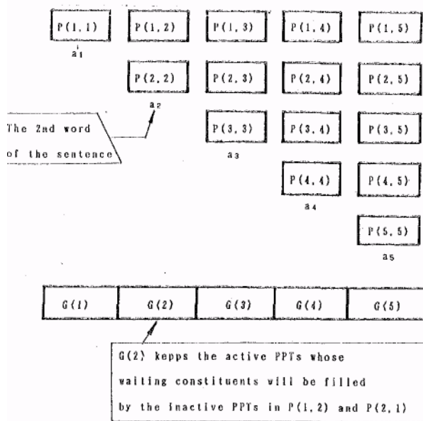
Fig. 2 Two Data Structures in KGW+p
