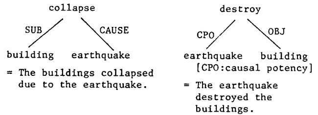
Fig. 11 An example of structural transformation in the generation phase.
