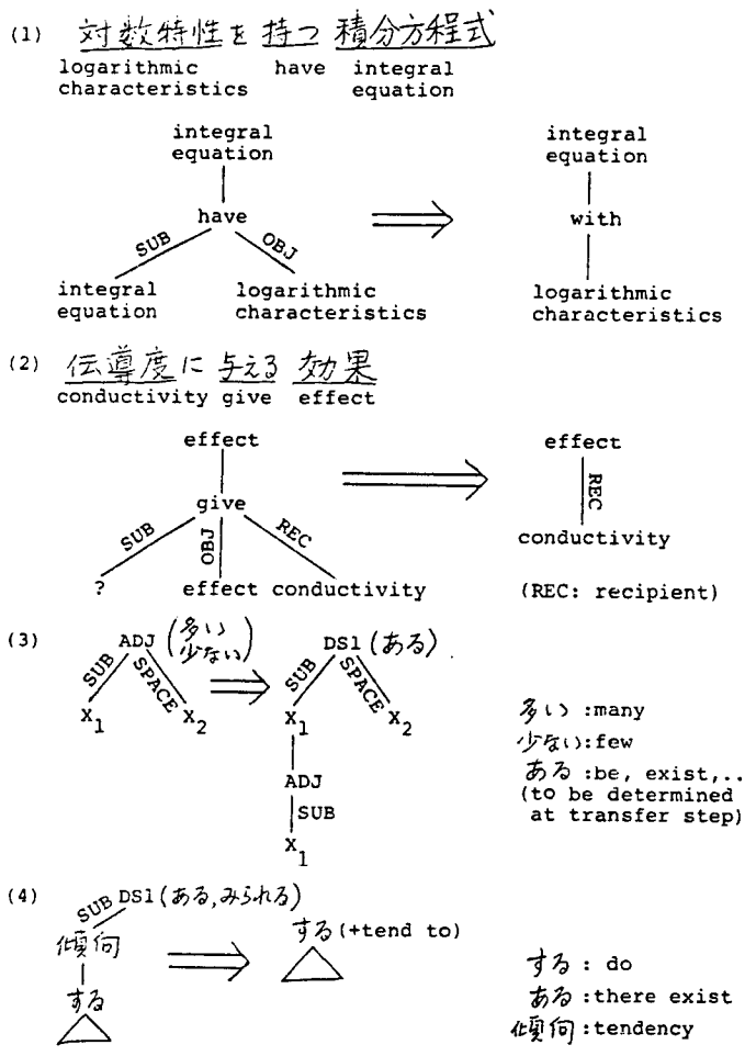
Fig. 5. An example of a heuristic rule used in the pre-transfer loop.
