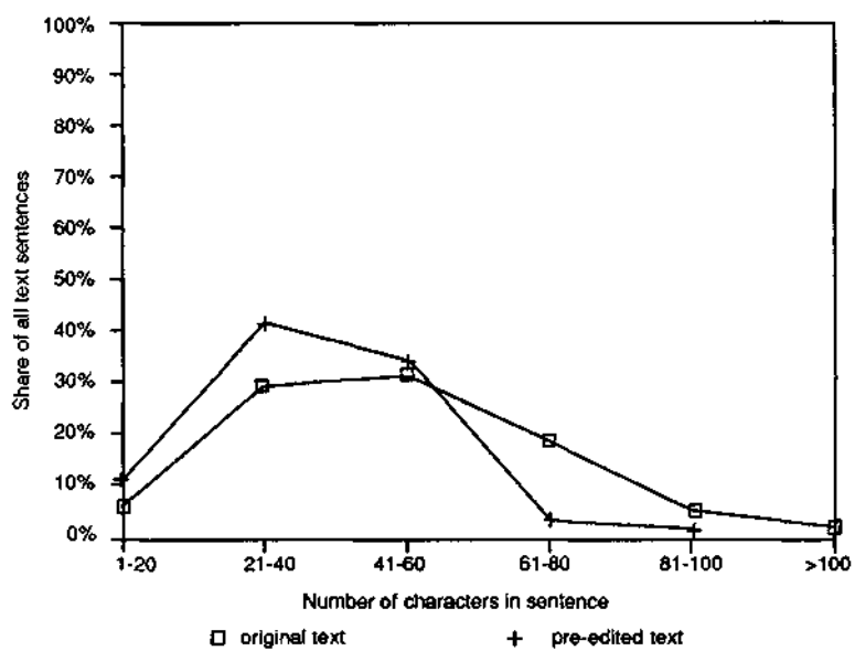
FIGURE 6 Length of sentences in text. SOURCE: Data collected by a major Japanese firm involved in machine translation development.
