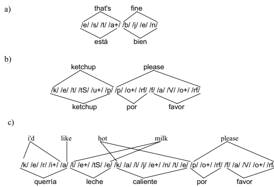
Fig. 1. Samples of alignments found by GIZA++
