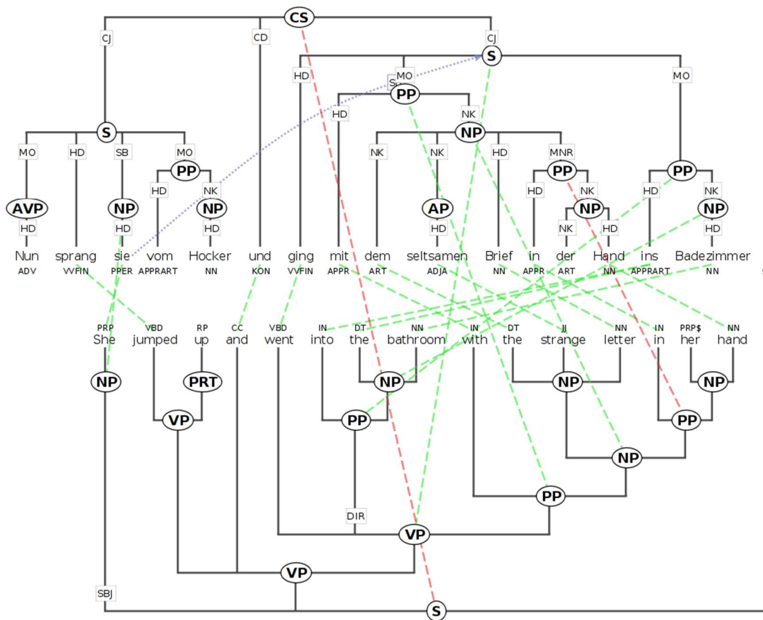
Figure 1: Tree pair German-English with word and phrase alignments.
